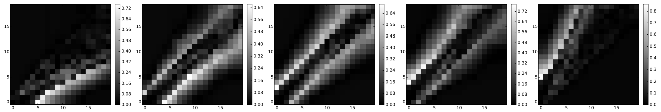
Figure 5. Absolute difference between value computed by AGPI- Q and the exact value. From left to right the error of the game (for player's budget = 0...20) for token's position 5 to 1
