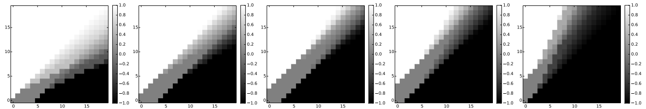
Figure 3. Exact value for the game of ALESIA. From left to right the value of the game (for player's budget = 0...20) for token's position 5 to 1
