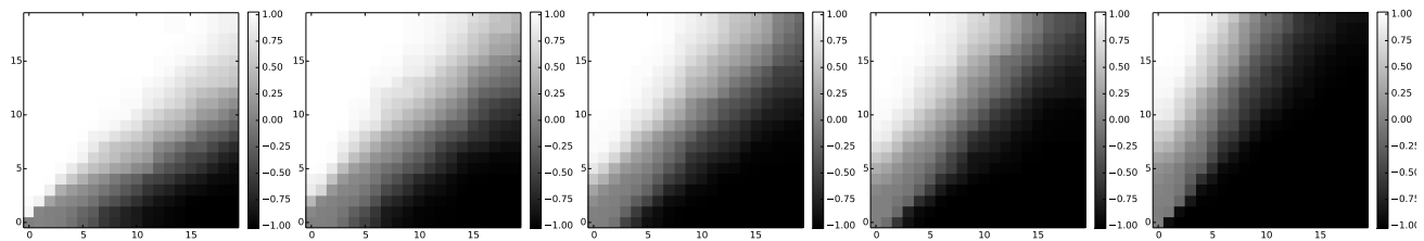
Figure 4. Value computed by AGPI-Q for the game of ALESIA. From left to right the approximate value of the game (for player's budget = 0...20) for token's position 5 to 1
